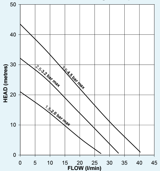
Monsoon Standard Single Pumps
