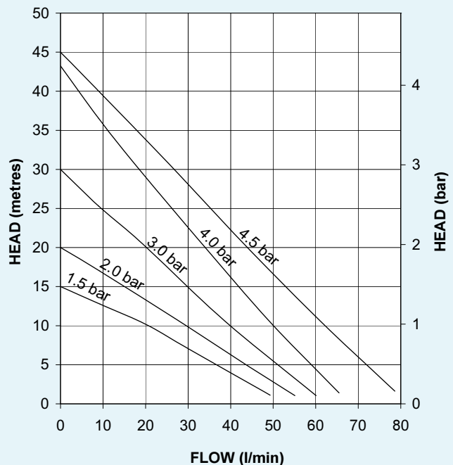
Monsoon Standard Twin Pumps
