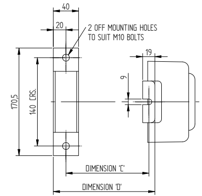
VIEW ON ARROW X MOUNTING FOOT DETAIL SCALE 12
